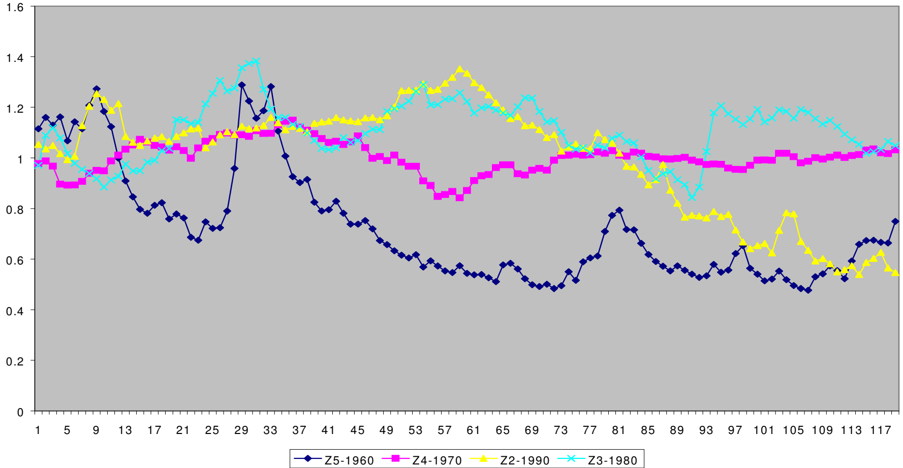
Figure 10: Comparison of Subsample Z(t)
